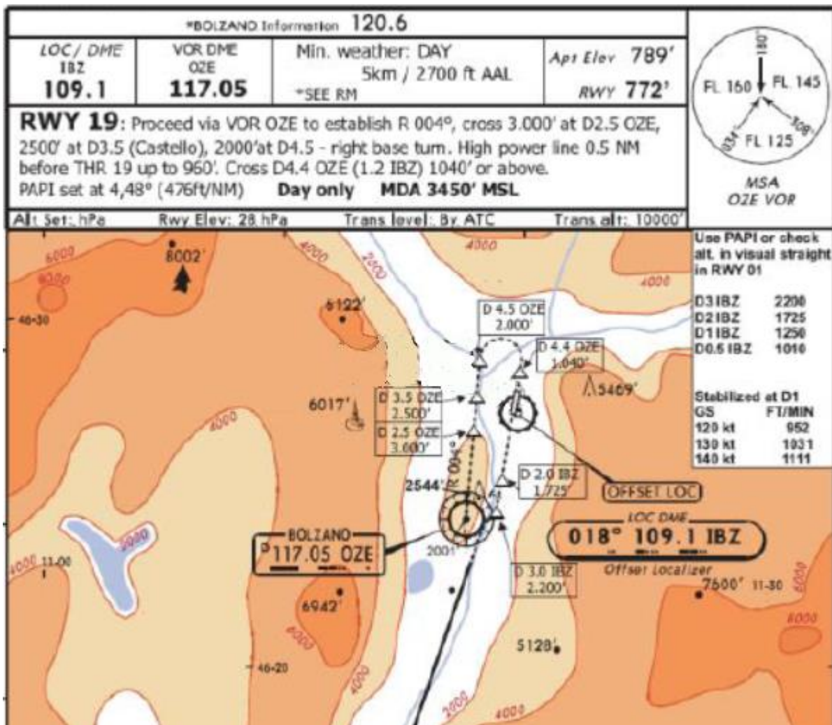
Figure 11: Visual part – straight in RWY 01 or right-hand traffic circuit after LOC + DME approach
