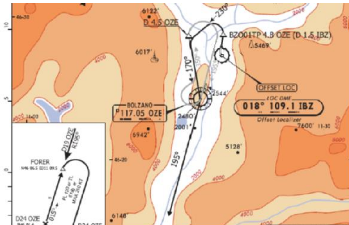
Figure 31: Sample for proposed take off contingency RWY01
