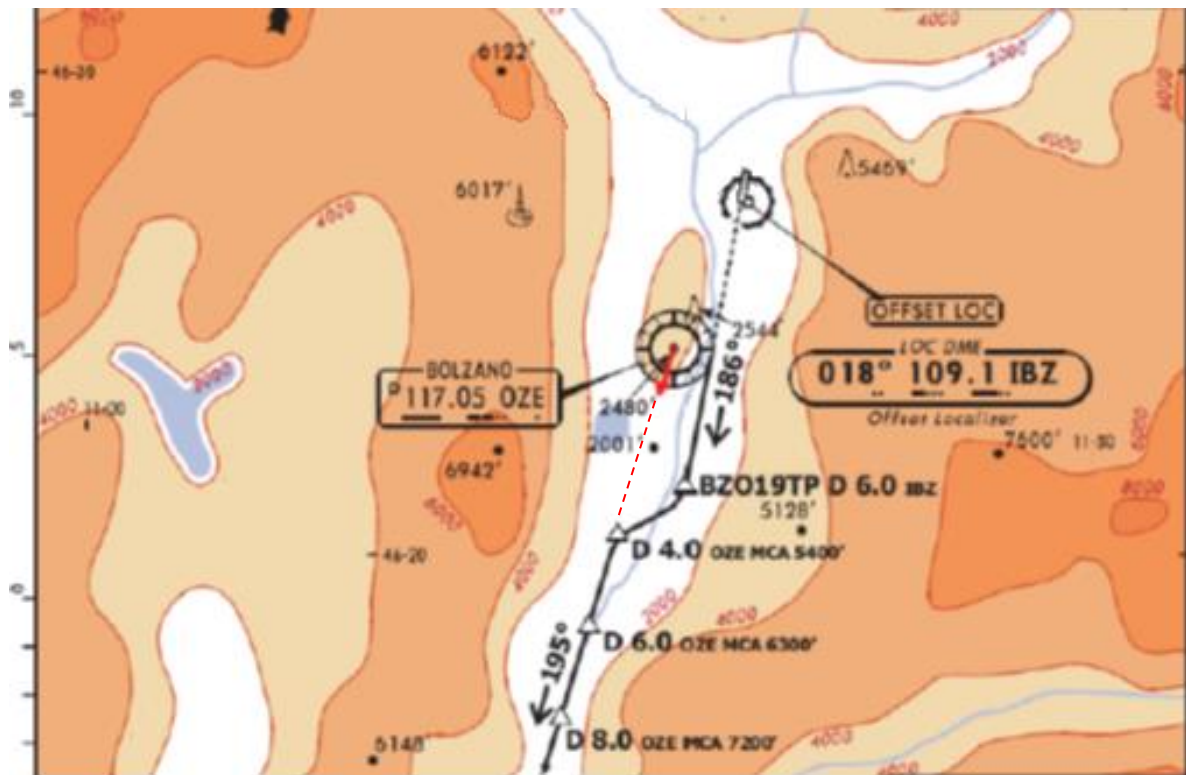
Figure 25: proposed all engine initial departure RWY 19
